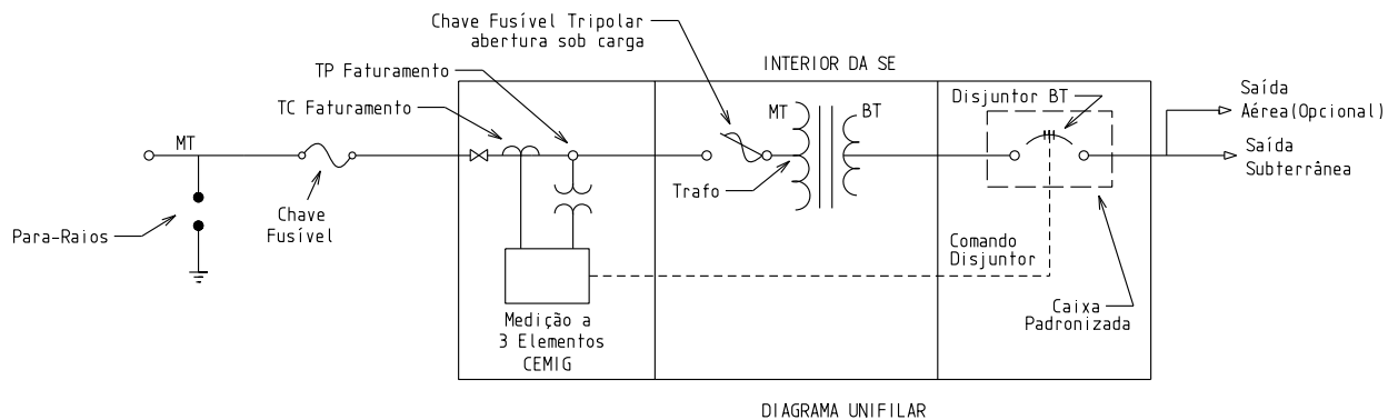
DIAGRAMA UNIFILAR
